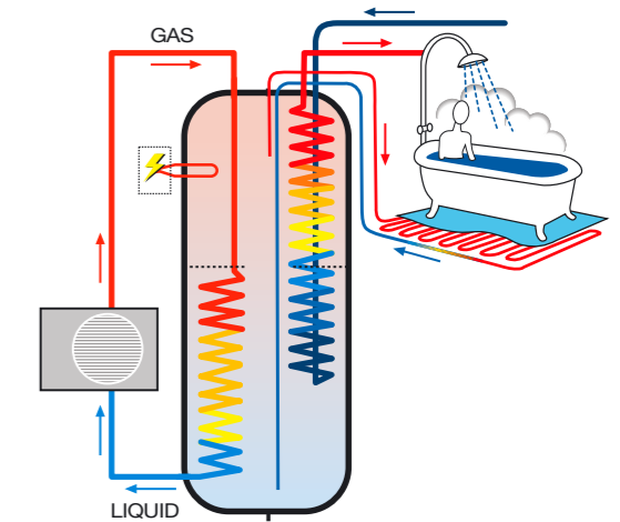
Energy transfer to the accumulator tank through the hot gas coil.
